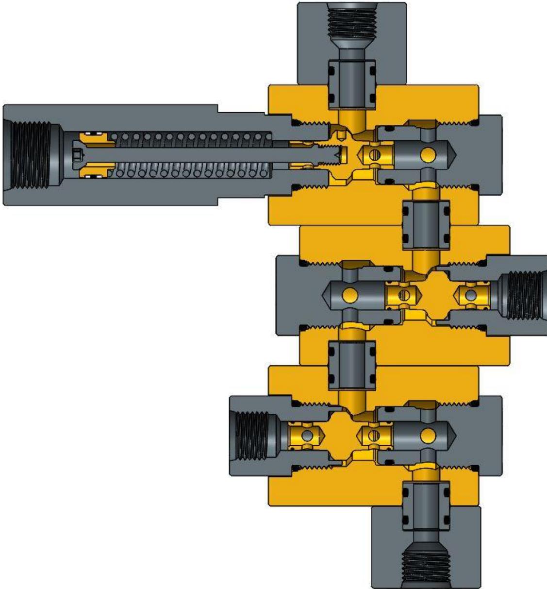
Figure 2. PN 29038: 1/2" MKIV Shuttle Valve, Stack, 4 Inlets, SAE, Pressure Biased, Low Interflow, High Drag
