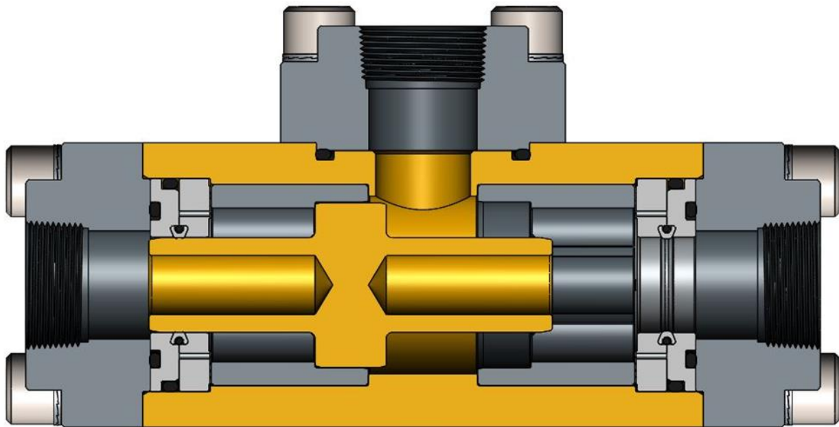
Figure 2. PN 29041: 1" NPT GEN 2 V-Seal Shuttle Valve, 3000 psi, High Interflow
