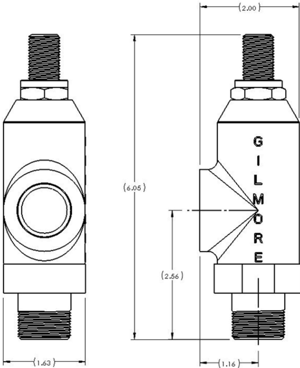
Figure 2. PN 25320-1 with cast bonnet PN 23401-2: Reference Dimensions
