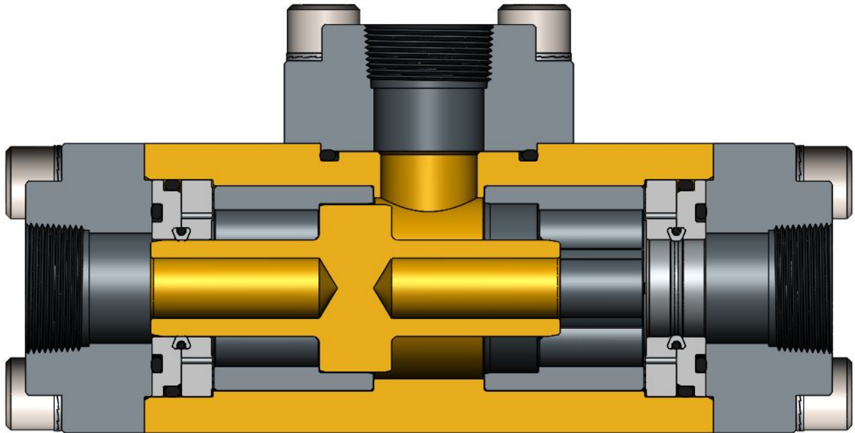
Figure 2. PN 29041: 1" NPT GEN 2 Shuttle Valve, 3000 psi, High Interflow
