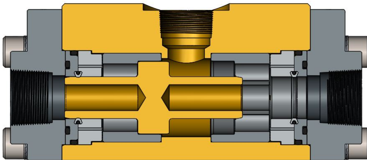
Figure 1. PN 29042: 1" NPT GEN 2 Shuttle Valve, 5000 psi, Low interflow
